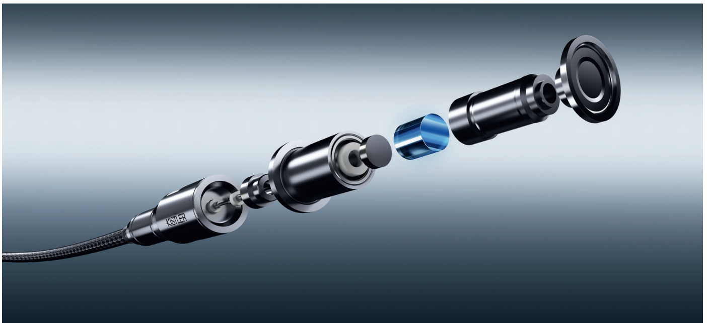
At the heart of the Kistler sensor technology is the crystal.
