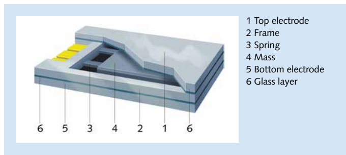
Fig. 9: MEMS variable capacitance accelerometer
