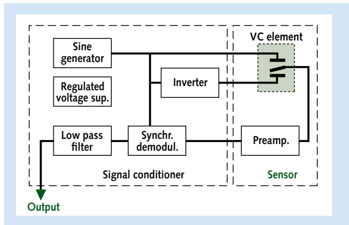
Fig. 8: Electrical schematic
