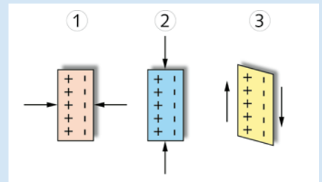
Fig. 3: Piezoelectric effect
