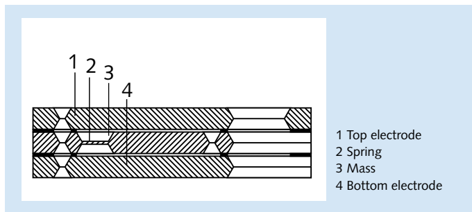
Fig. 7: Typical capacitive accelerometer arrangement
