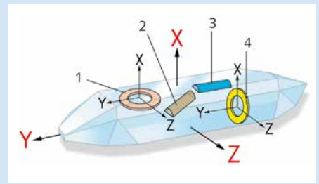
Fig. 2: Quartz bar
